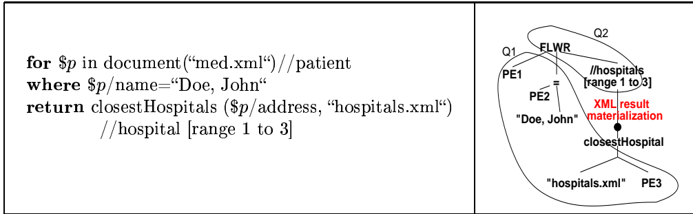
Figure 13: Query necessitating intermediate XML result materialization
